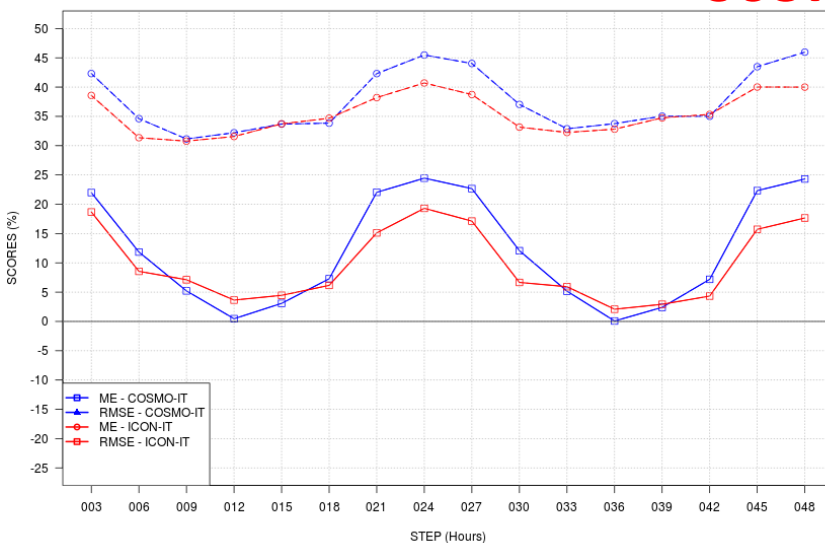
SCORES vs STEP - TCC - JJA 2024 - ALL ITA stations ALL
