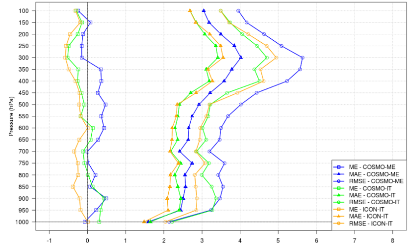
SCORES - WSpeed - SON 2024 - All ITA TEMP stations - step048
