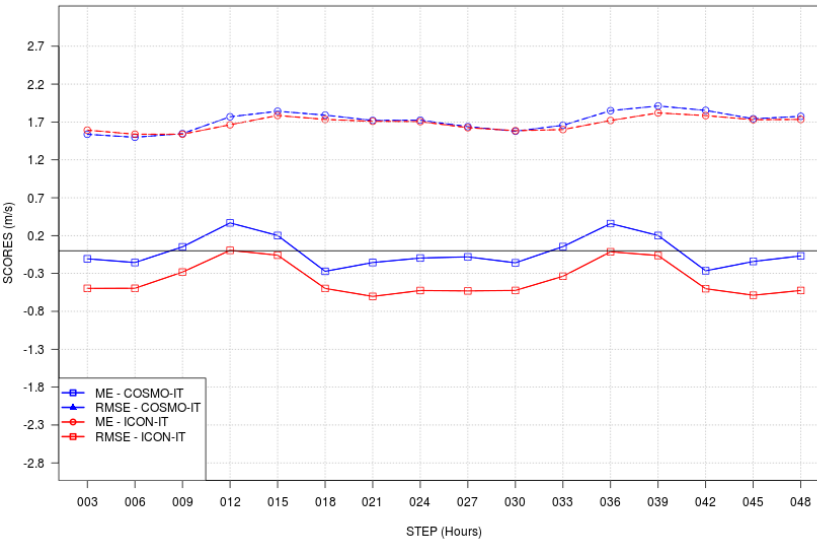
SCORES vs STEP - WS - JJA 2024 - ALL ITA stations
