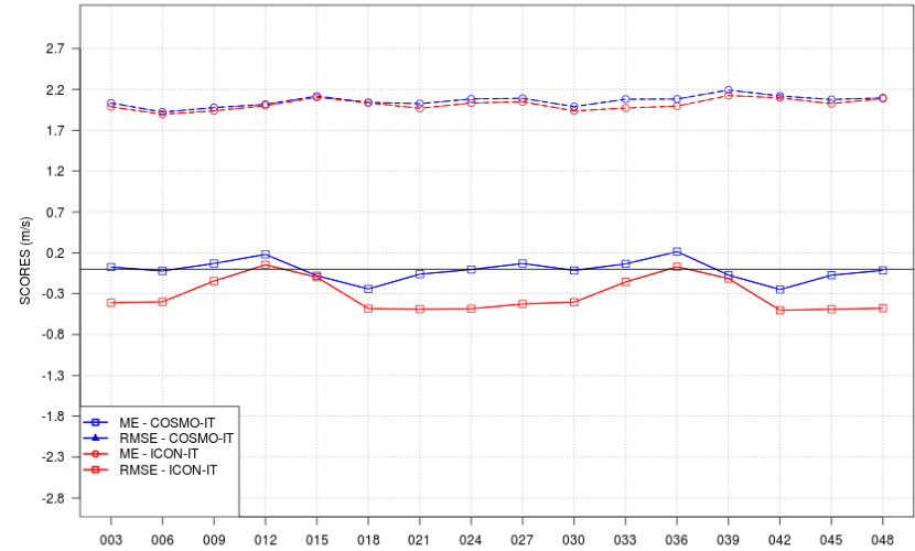
SCORES vs STEP - WS - SON 2024 - ALL ITA stations
