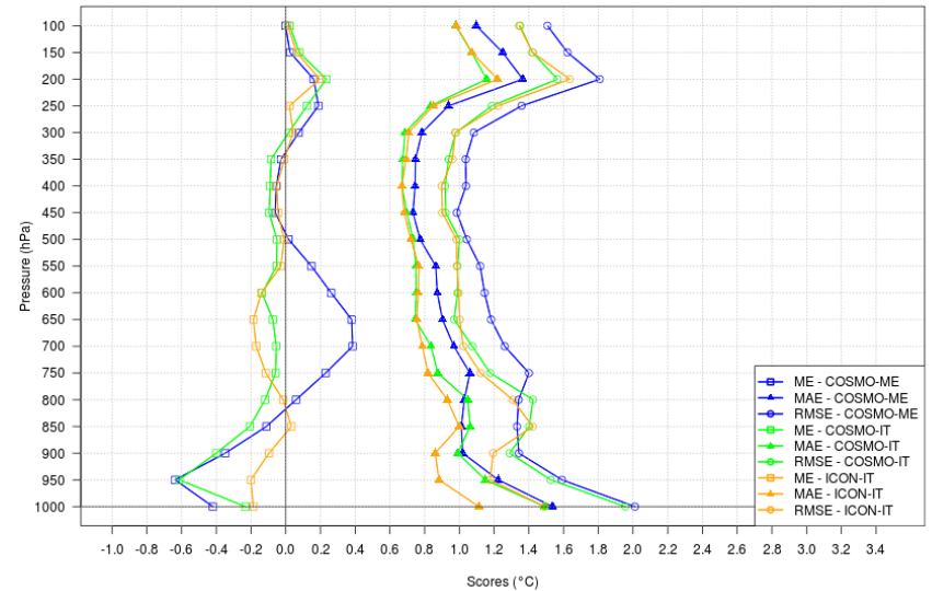
SCORES - T - SON 2024 - All ITA TEMP stations - step048
