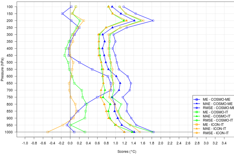
SCORES - T - JJA 2024 - All ITA TEMP stations - step048
