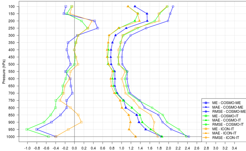
SCORES - T - JJA 2024 - All ITA TEMP stations - step048
