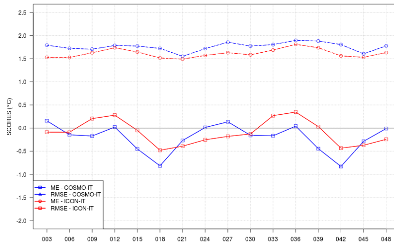
SCORES vs STEP - T2M - SON 2024 - ALL ITA stations ALL
