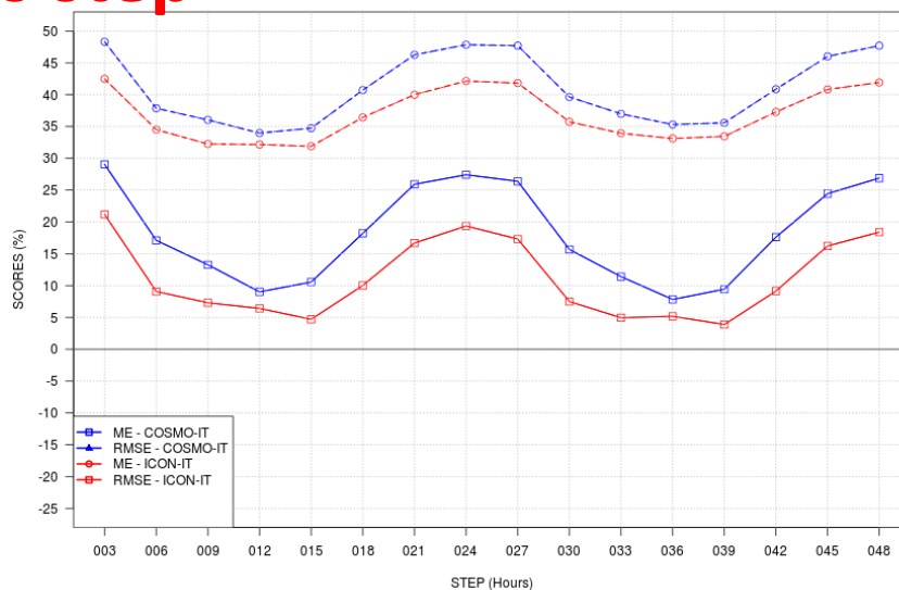
SCORES vs STEP - TCC - SON 2024 - ALL ITA stations ALL
