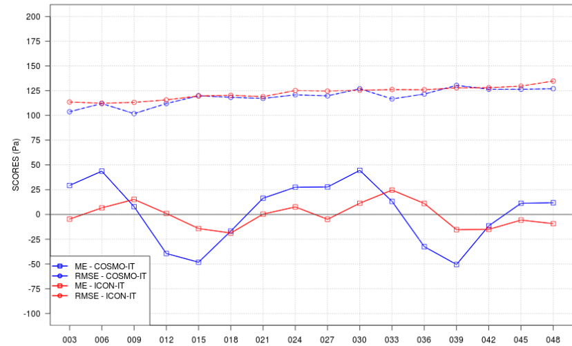
SCORES vs STEP - PS - SON 2024 - ALL ITA stations ALL
