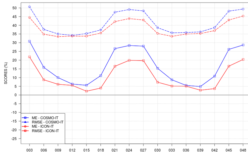
SCORES vs STEP - TCC - SON 2024 - ALL ITA stations ALL
