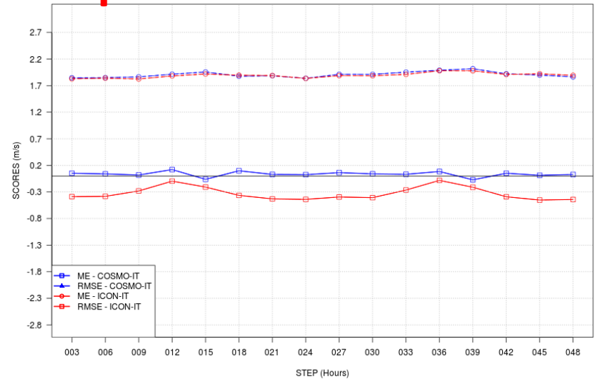
SCORES vs STEP - WS - SON 2024 - ALL ITA stations
