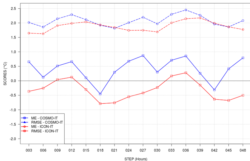
SCORES vs STEP - T2M - JJA 2024 - ALL ITA stations ALL
