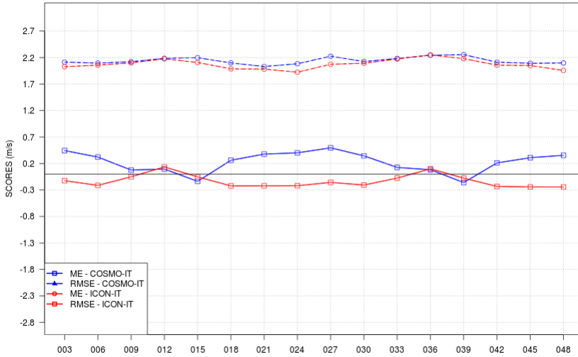
SCORES vs STEP - WS - JJA 2024 - ALL ITA stations
