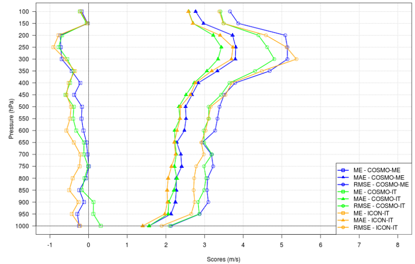
SCORES - WSpeed - SON 2024 - All ITA TEMP stations - step048
