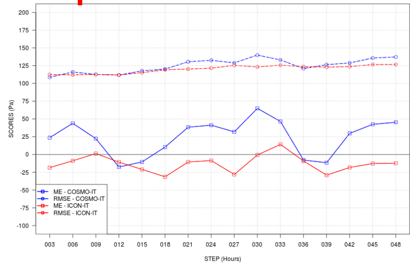
SCORES vs STEP - PS - SON 2024 - ALL ITA stations ALL
