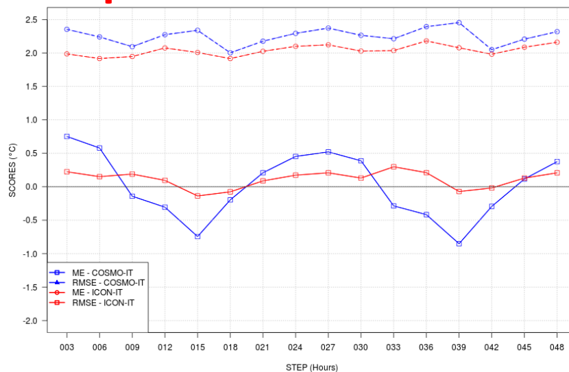
SCORES vs STEP - T2M - SON 2024 - ALL ITA stations ALL
