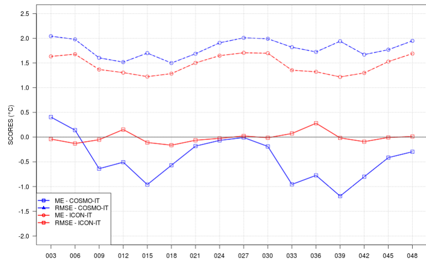
SCORES vs STEP - T2M - JJA 2024 - ALL ITA stations ALL
