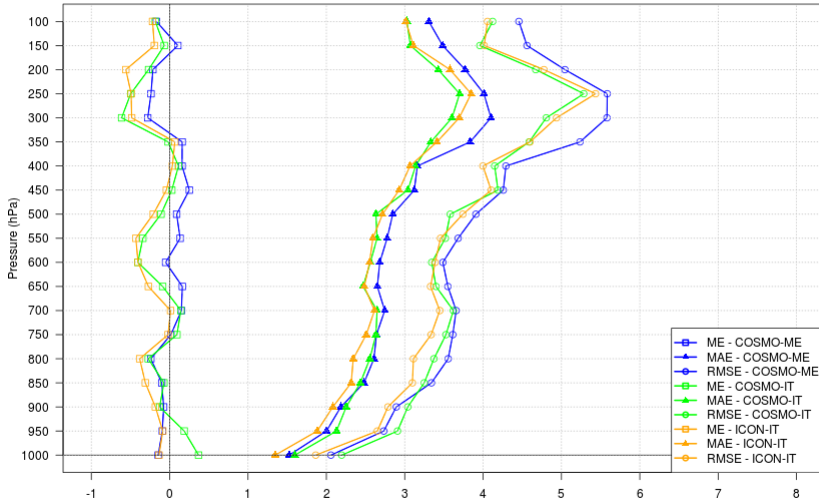
SCORES - WSpeed - JJA 2024 - All ITA TEMP stations - step048
