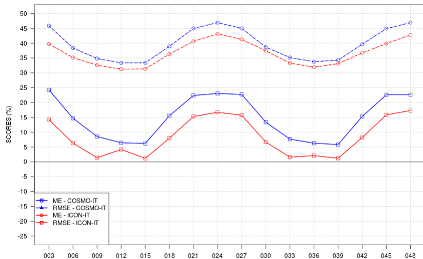
SCORES vs STEP - TCC - JJA 2024 - ALL ITA stations ALL
