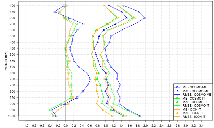
SCORES - T - SON 2024 - All ITA TEMP stations - step048
