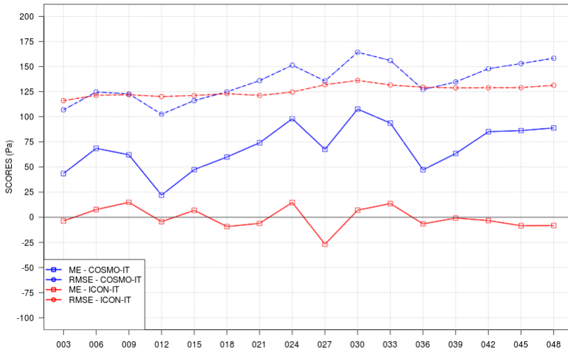
SCORES vs STEP - PS - JJA 2024 - ALL ITA stations ALL
