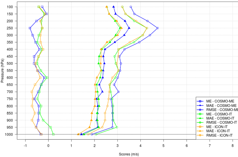
SCORES - WSpeed - JJA 2024 - All ITA TEMP stations - step048
