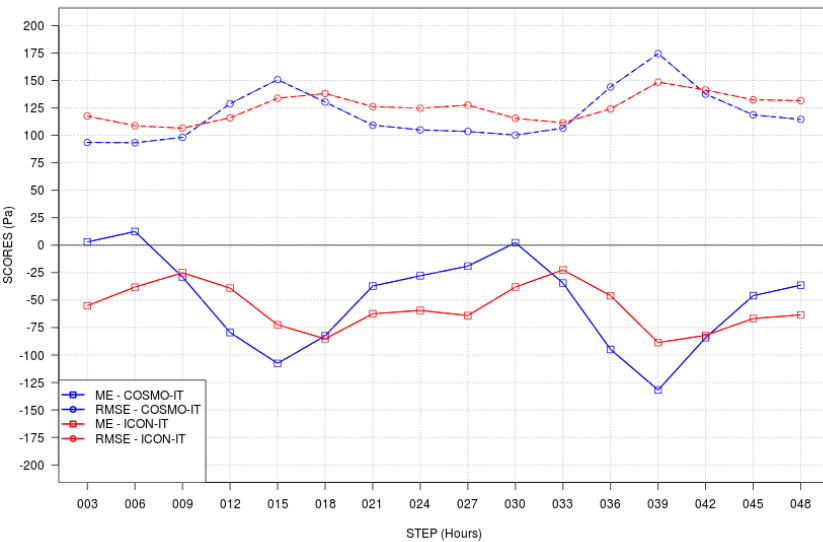
SCORES vs STEP - PS - JJA 2024 - ALL ITA stations ALL
