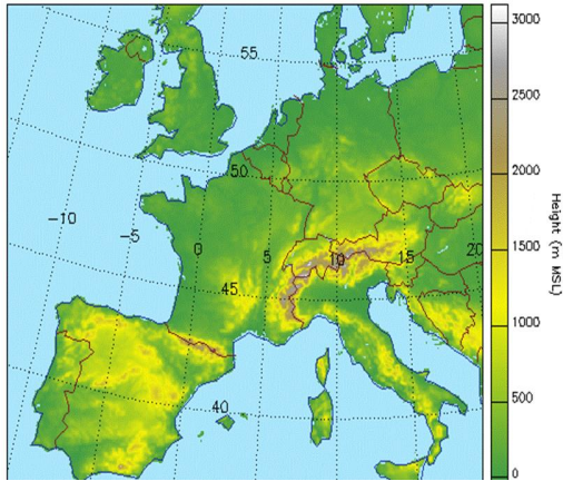
Geographical domain of the (old) weather prediction system used at Meteoswiss
