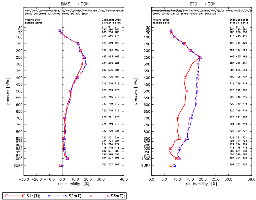
FIGURE 5-2. Bias (left panel) and standard deviation (right panel) of the relative humidity at initialization time calculated for the 27 forecasts against the 28 stations defined in section 5.1. Red curves are for observing system S1, blue curves for observing system S2 and magenta curves for observing system S3.
