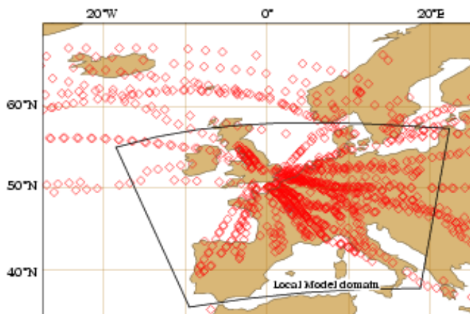
FIGURE 4-1. Typical daily coverage of activated AMDAR platforms in observing system S3 (red boxes).
