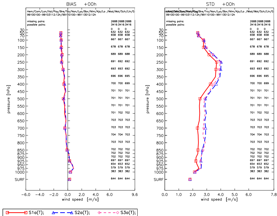
FIGURE 5-4. Bias (left panel) and standard deviation (right panel) of the wind speed at initialization time calculated for the 27 forecasts against the 28 stations defined in section 5.1. Red curves are for observing system S1, blue curves for observing system S2 and magenta curves for observing system S3.
