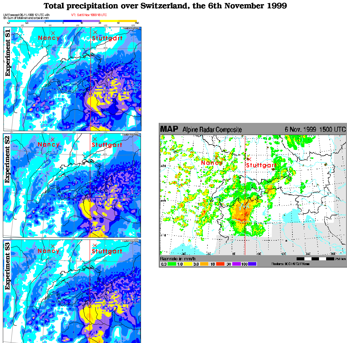
FIGURE 5-13. Sensitivity of a heavy precipitation event over Southern part of the Alps to the observing system. Left panels: 6 hours sum of total precipitation forecast over Switzerland, evaluated on the 6th November 1999 between 12 UTC (analysis time) and 18 UTC. Right panel: Total precipitation rate observed by the MAP Alpine Radar Composite on the 6th November 1999 at 15 UTC (data for the whole MAP period are available on-line at www.map.ethz.ch ). Yellow areas in the left panels can be compared with light orange areas in the right panel, and correspond to about 20 to 50 mm precipitation in 6 hours.
