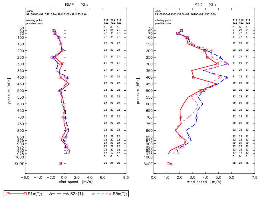
FIGURE 5-9. As in figure 5-8, for wind speed.
