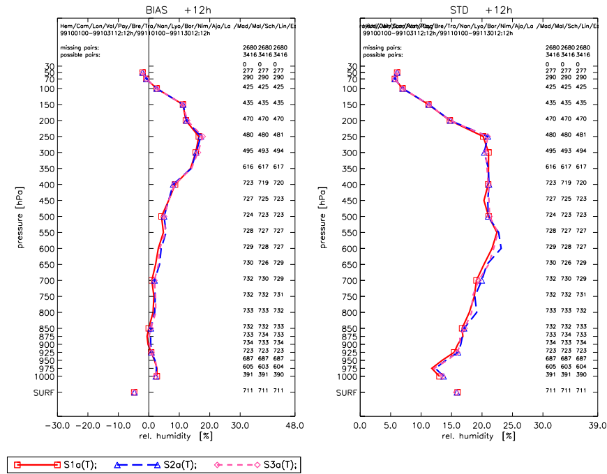
FIGURE 5-3. As in figure 5-2, after 12 hour forecast.
