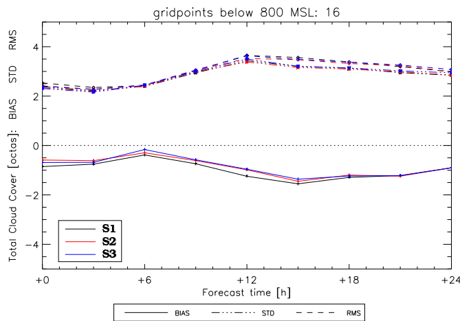
FIGURE 5-11. As figure 5-10, for the total cloud cover verified against the 16 active ANETZ stations associated to a model grid point below 800 m. All grid points within 30 km of an observation location are considered when calculating the scores.
