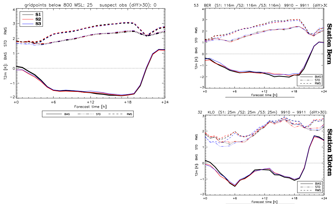
FIGURE 5-13. Upper left panel: hourly variation of bias (solid line) and standard deviation (dashed line) for the 2-m temperature, verified against the 25 active ANETZ stations associated to a model grid point below 800 m. Black curves are for observing system S1, red curves for observing system S2 and blue curves for observing system S3. Right panels: same as upper left panel but for a single ANETZ station. Both Bern and Kloten are on the Swiss Plateau, the latter one is also at an international airport location.
