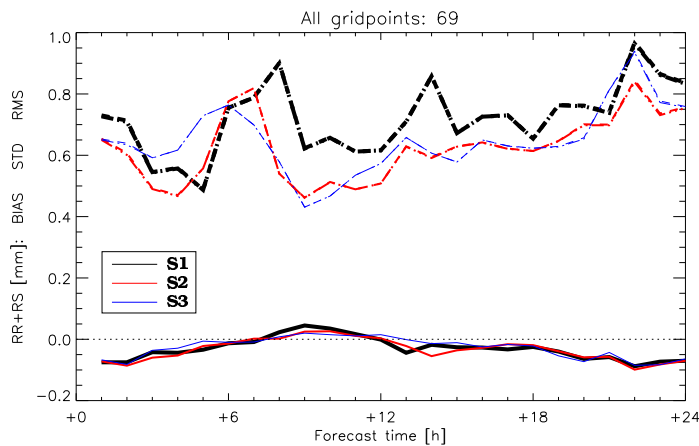
FIGURE 5-12. As figure 5-10, for the hourly total precipitation verified against all 69 active ANETZ stations. The plain lines represent the bias, the dash/dotted lines the standard deviation. A mean of 5 grid points around an observation is done before calculating the scores.
