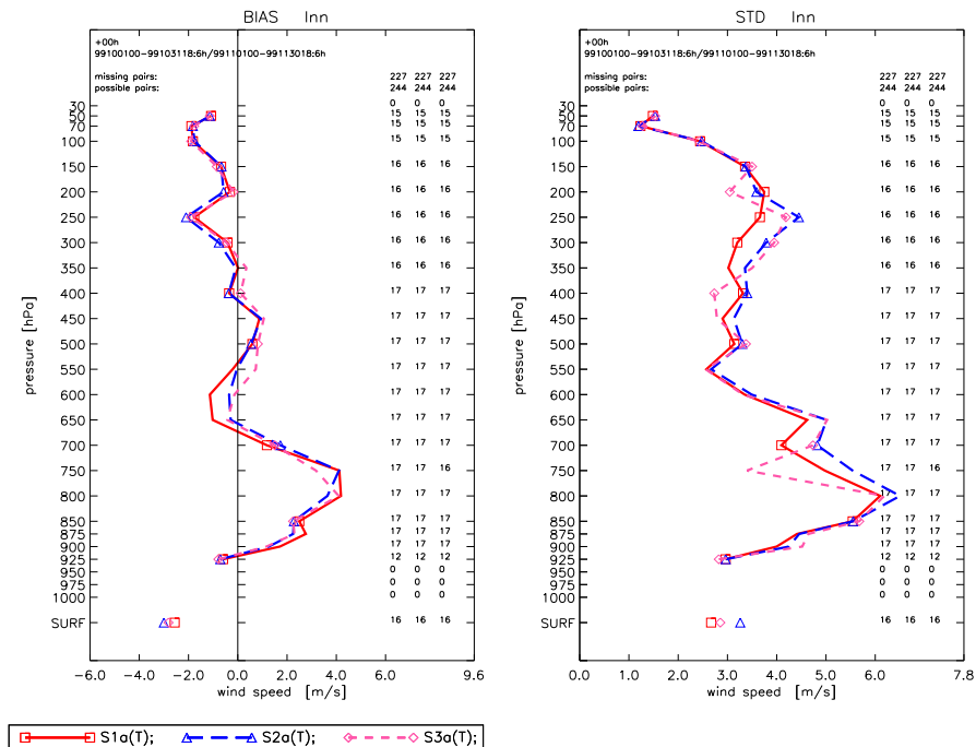
FIGURE 5-6. Bias (left panel) and standard deviation (right panel) of the wind speed at initialization time calculated for the 27 forecasts against the vertical sounding at Innsbruck. Red curves are for observing system S1, blue curves for observing system S2 and magenta curves for observing system S3. Innsbruck is a radiosonde station which is not used in our OSE.
