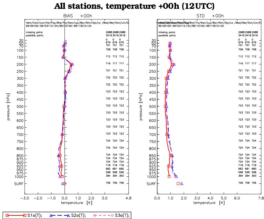
FIGURE 5-1. Bias (left panel) and standard deviation (right panel) of the temperature at initialization time calculated for the 27 forecasts against the 28 stations defined in section 5.1. Red curves are for observing system S1, blue curves for observing system S2 and magenta curves for observing system S3.
