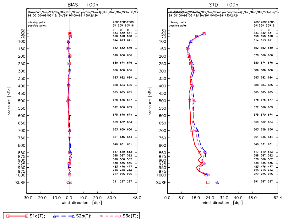
FIGURE 5-5. As in figure 5-4, for the wind direction.
