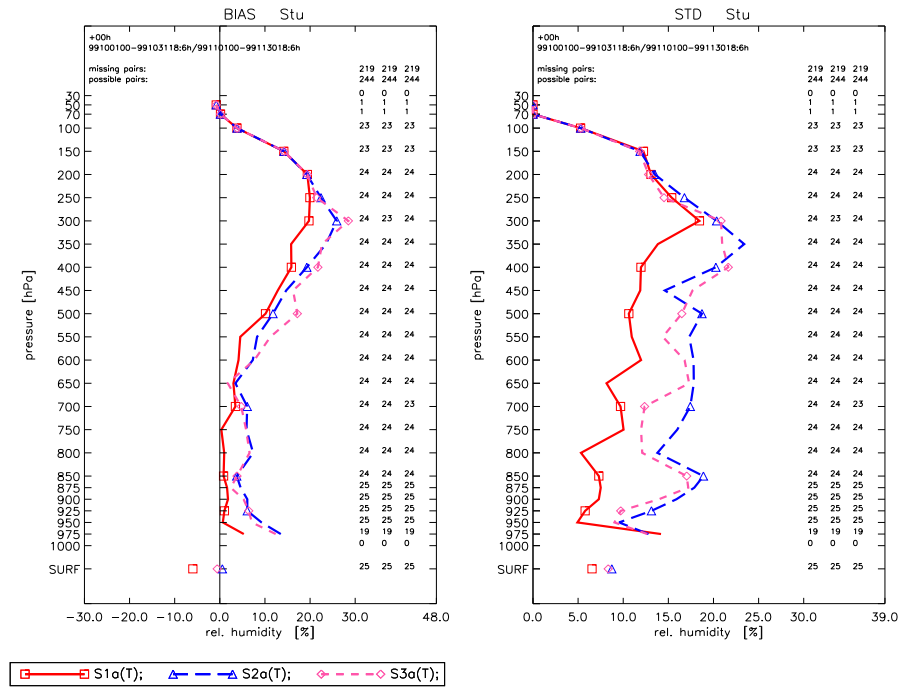
FIGURE 5-8. Bias (left panel) and standard deviation (right panel) of the relative humidity at initialization time calculated for the 27 forecasts against the vertical sounding at Stuttgart. Red curves are for observing system S1, blue curves for observing system S2 and magenta curves for observing system S3. Stuttgart is a radiosonde station which is blacklisted in S2 and S3, and is a location with many AMDARs data.
