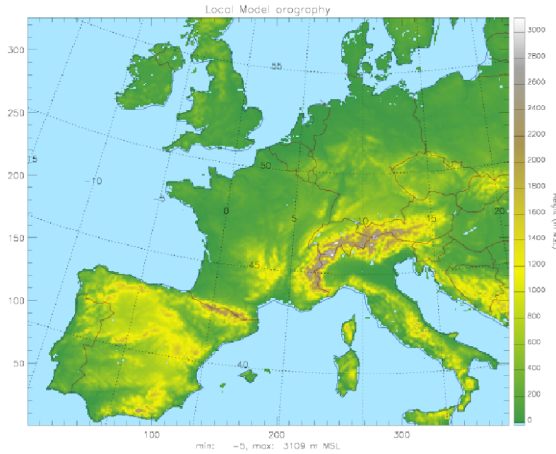
FIGURE 2-1. Domain and orography of aLMo (min: - 5 m, max: 3109 m).
