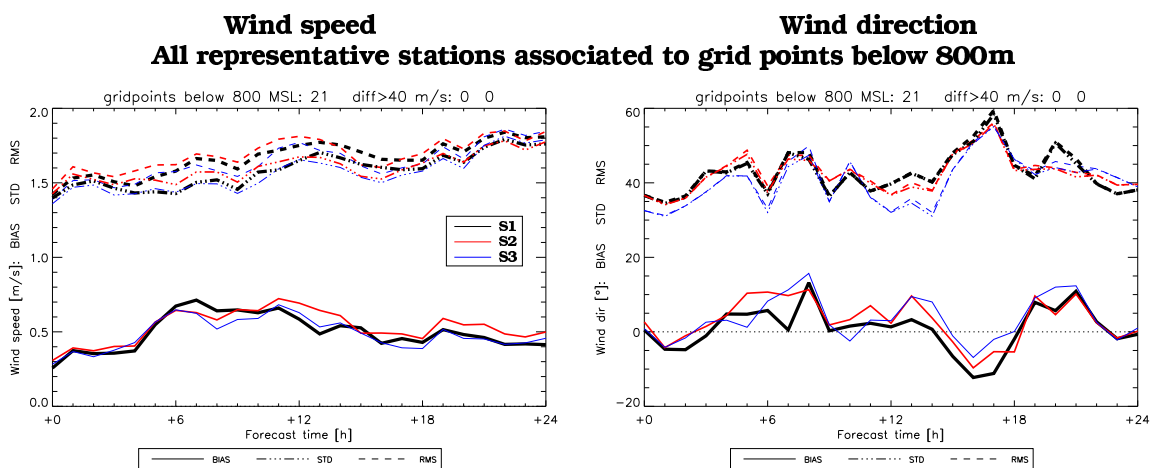
FIGURE 5-10. Hourly variation of some statistical scores for the 10-m wind speed (left panel) and for the 10-m wind direction (right panel), verified against the 21 representative ANETZ stations associated to a model grid point below 800 m. Black curves are for observing system S1, red curves for observing system S2 and blue curves for observing system S3. The plain lines represent the bias, the dotted lines represent the rms and the dash/dotted lines represent the standard deviation.
