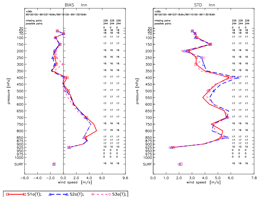
FIGURE 5-7. As in figure 5-6, after 6 hour forecast.
