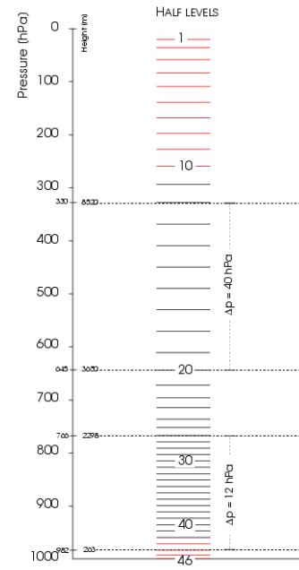
FIGURE 2-2. Vertical distribution of layers in aLMo.
