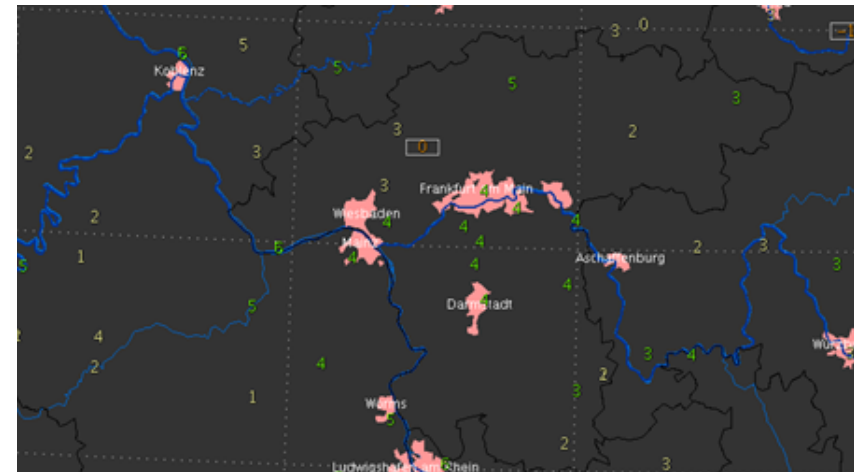
2m temperature
