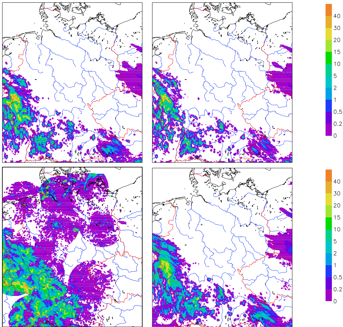
Figure 4: Simulated 23-hour precipitation sums (in mm) of LMK forecasts started 2004-08-07 00 UTC. Upper left: N_0^g = 4 \times 10^6 \text{ m}^{-4} , \rho_g \approx 0.2 \text{ g/cm}^3 ; upper right: N_0^g = 4 \times 10^4 \text{ m}^{-4} , \rho_g = 0.9 \text{ g/cm}^3 ; lower right: no graupel (standard LM microphysics). Lower left: corresponding radar-derived precipitation observation.
