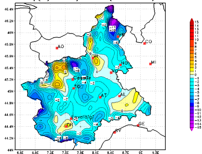
2m Mean Temp(°C) Monthly Anom. (1971–2000) in JUL2011
