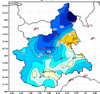
Monthly precipitation diff. (obs-med) in mm at JUL2011 Climatological period 1971–2000
