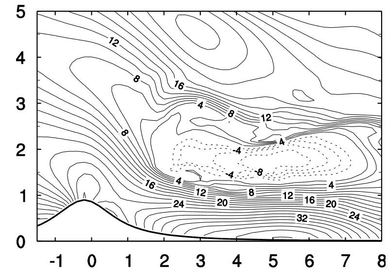
CE-C-Implicit
