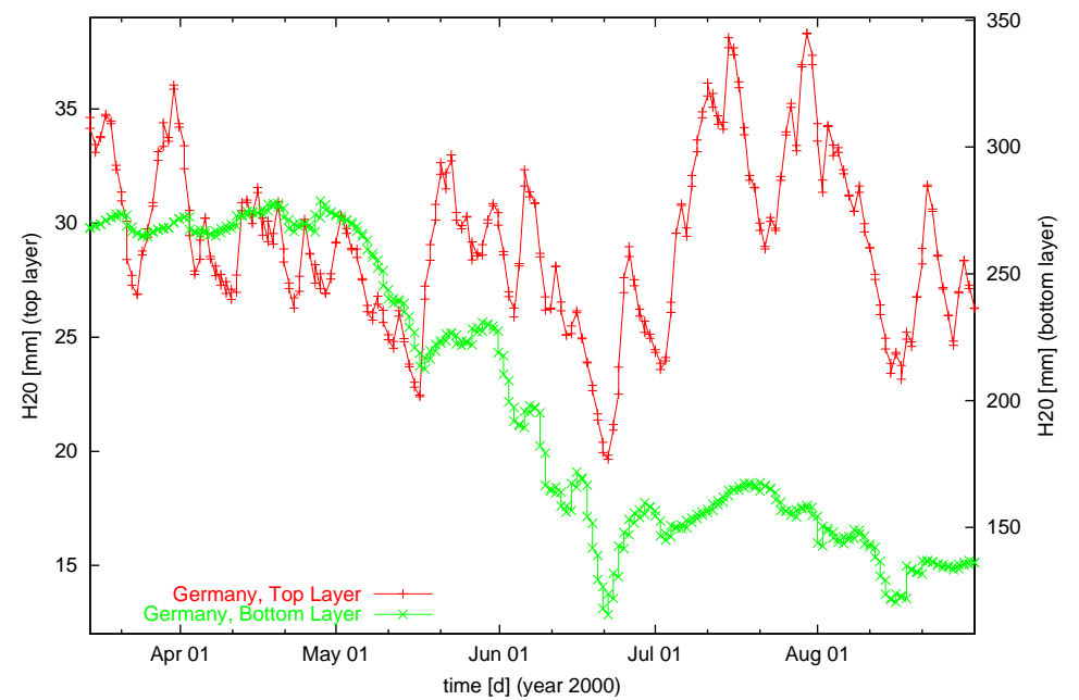
Soil Moisture Increments (SMA)
