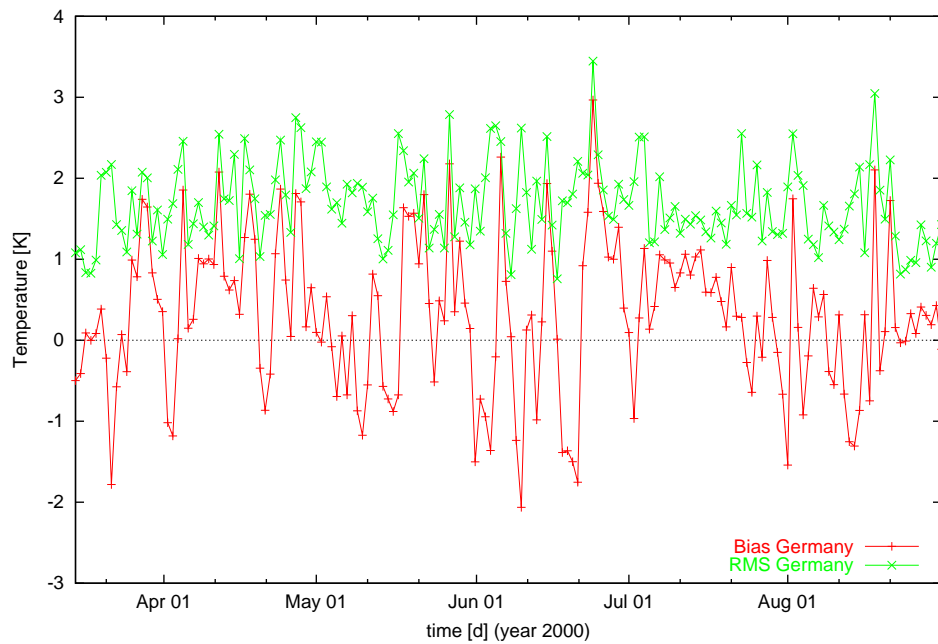
T2m Forecast Errors (SMA)
