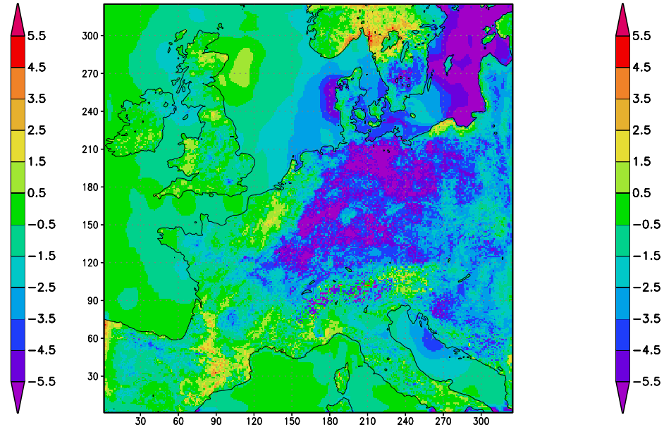
T2m Forecast Error [K], Jun 21, 2000
