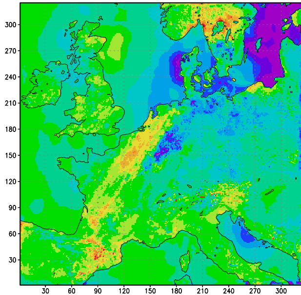
T2m Forecast Error [K], jun 21, 2000
