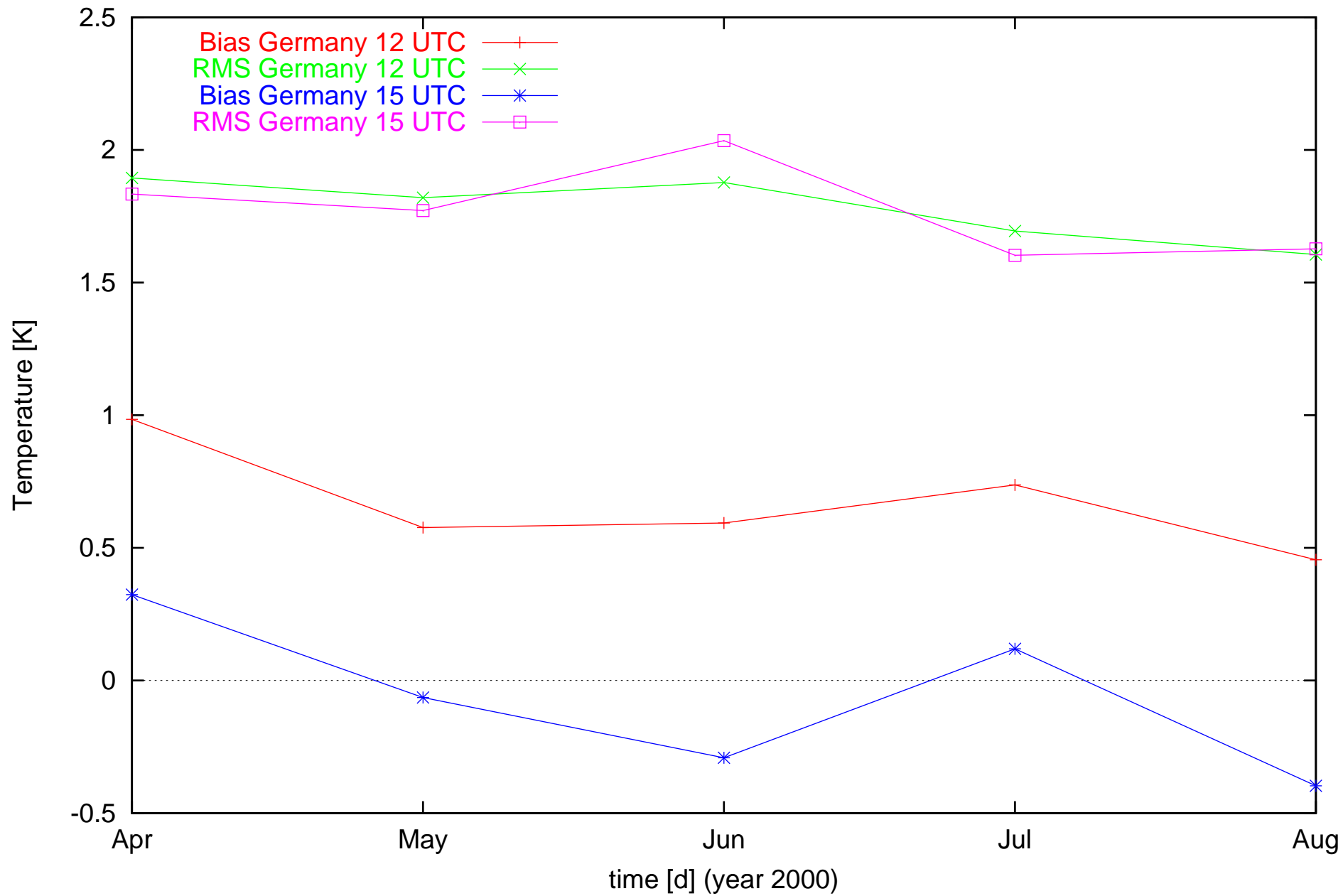
T2m Forecast Errors (SMA)
